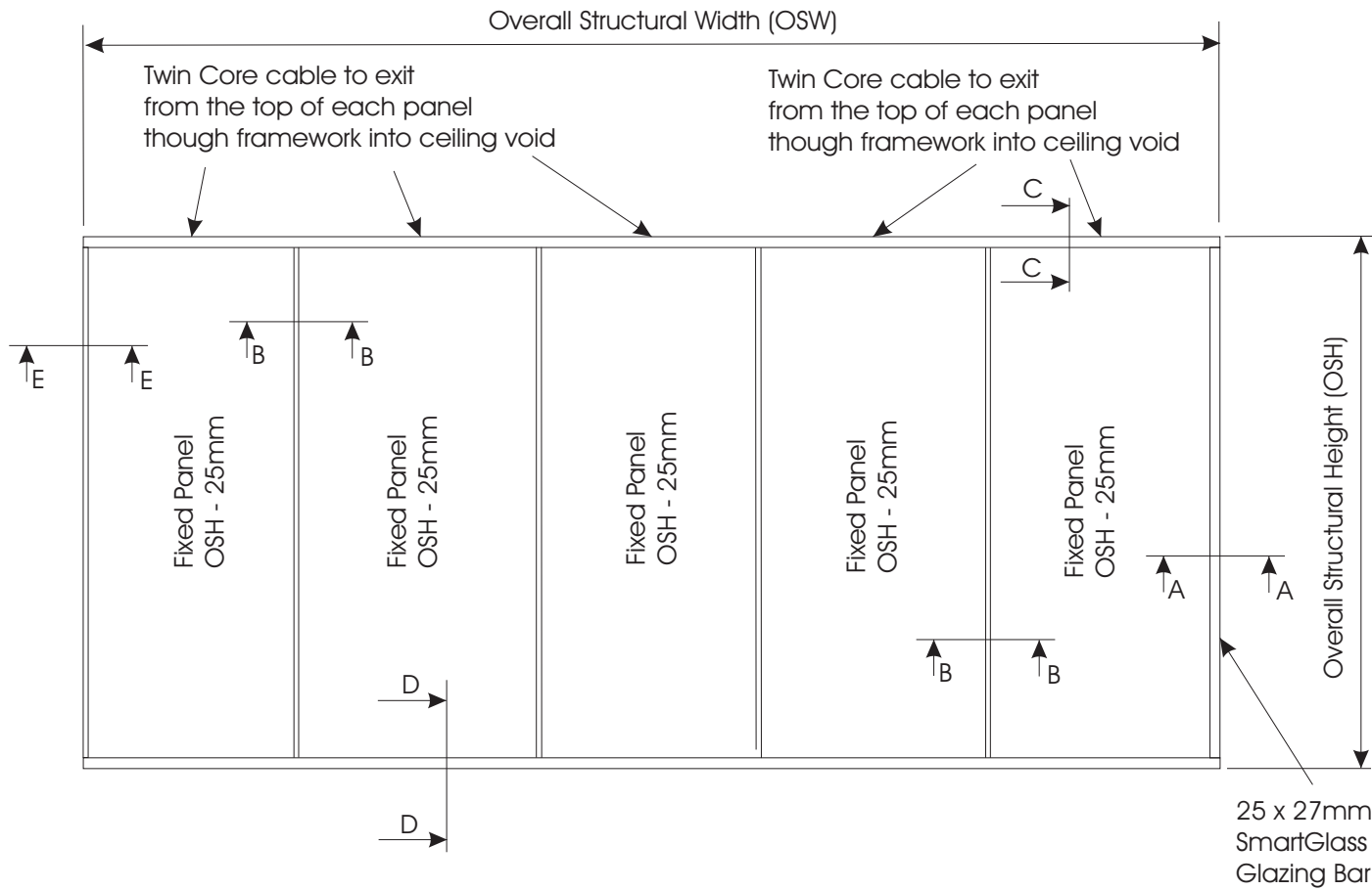
Side Elevation
